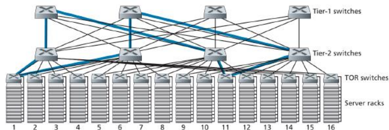
شکل ۳: Highly interconnected data center network
